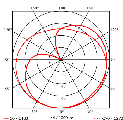
F31750_8W_LED_IC_S1
